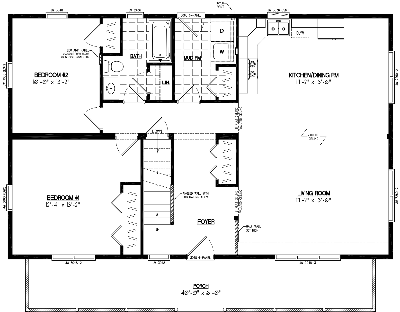
28x44 MOUNTAINEER DELUXE Plan #28MD1404
