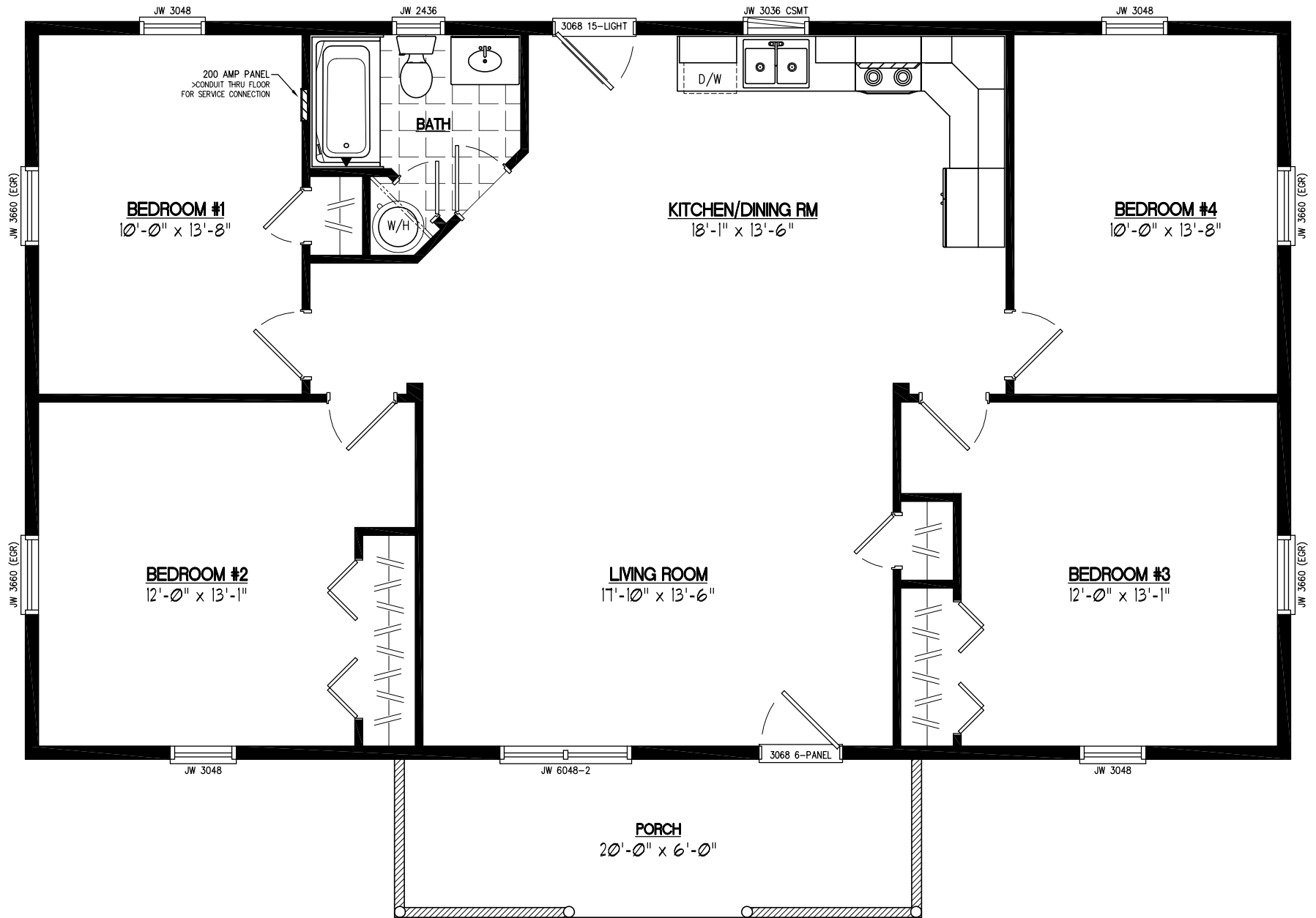
28x48 PIONEER Plan #28PR1204
