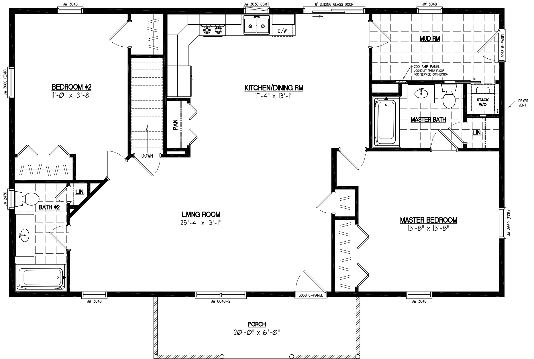
28x48 PIONEER Plan #28PR1205
