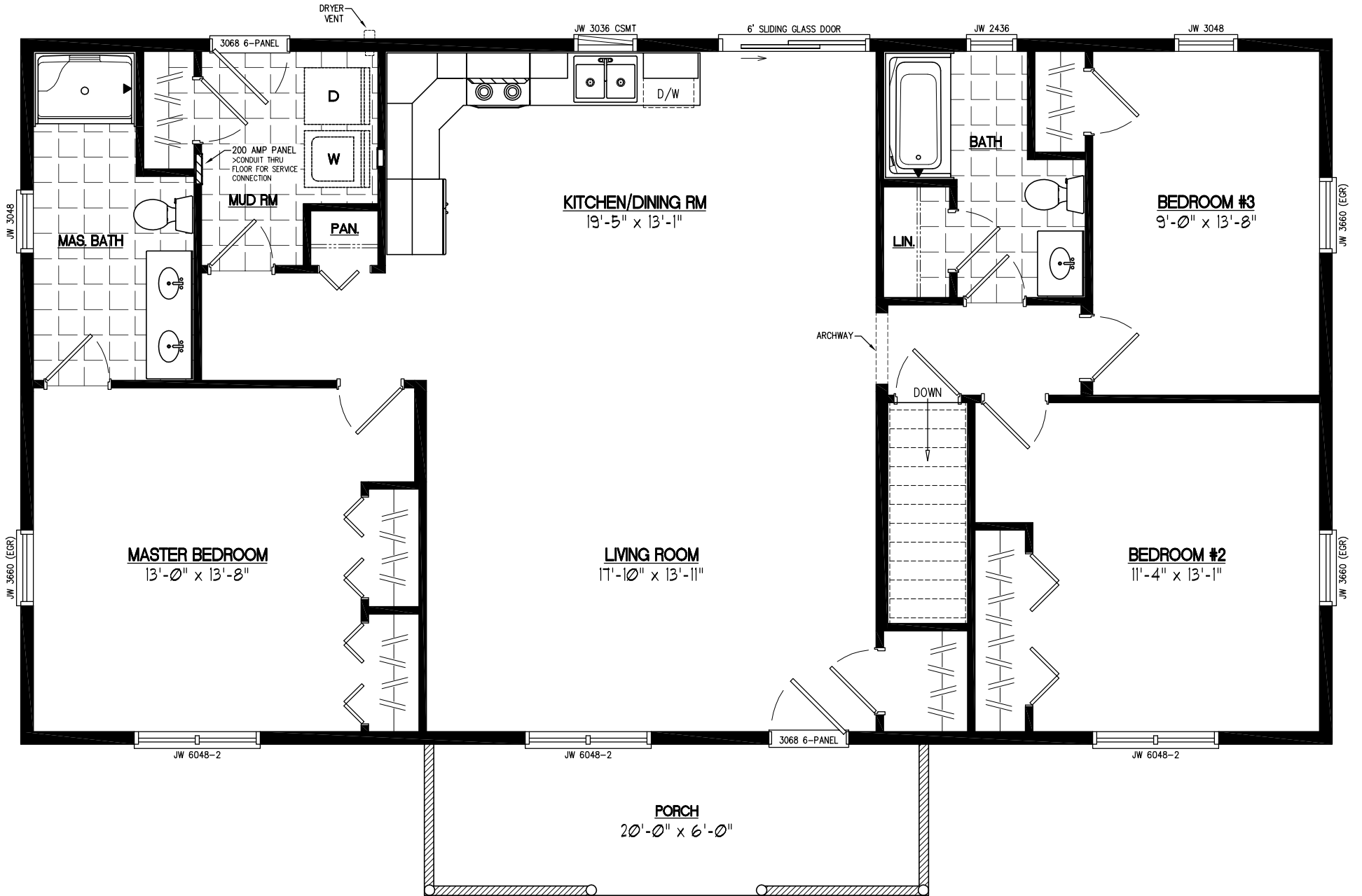
28x52 PIONEER Plan #28PR1207
