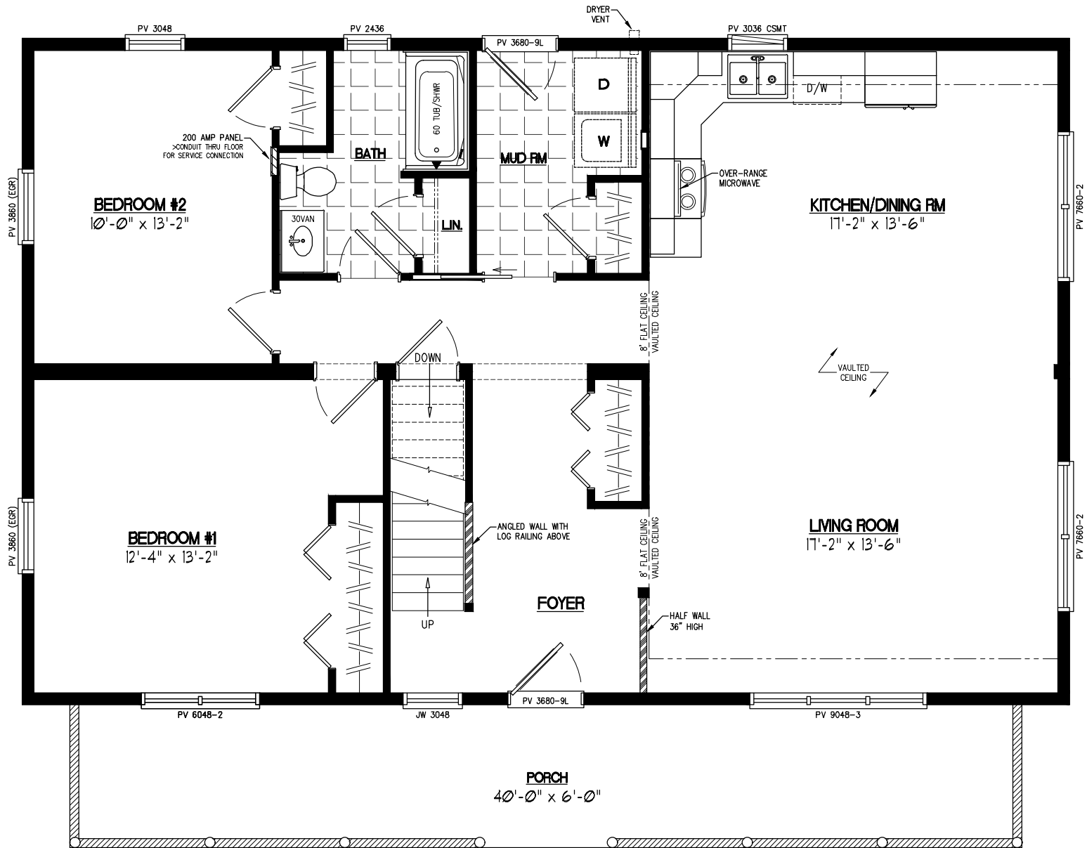
28x44 MOUNTAINEER DELUXE Plan #28MD1404
