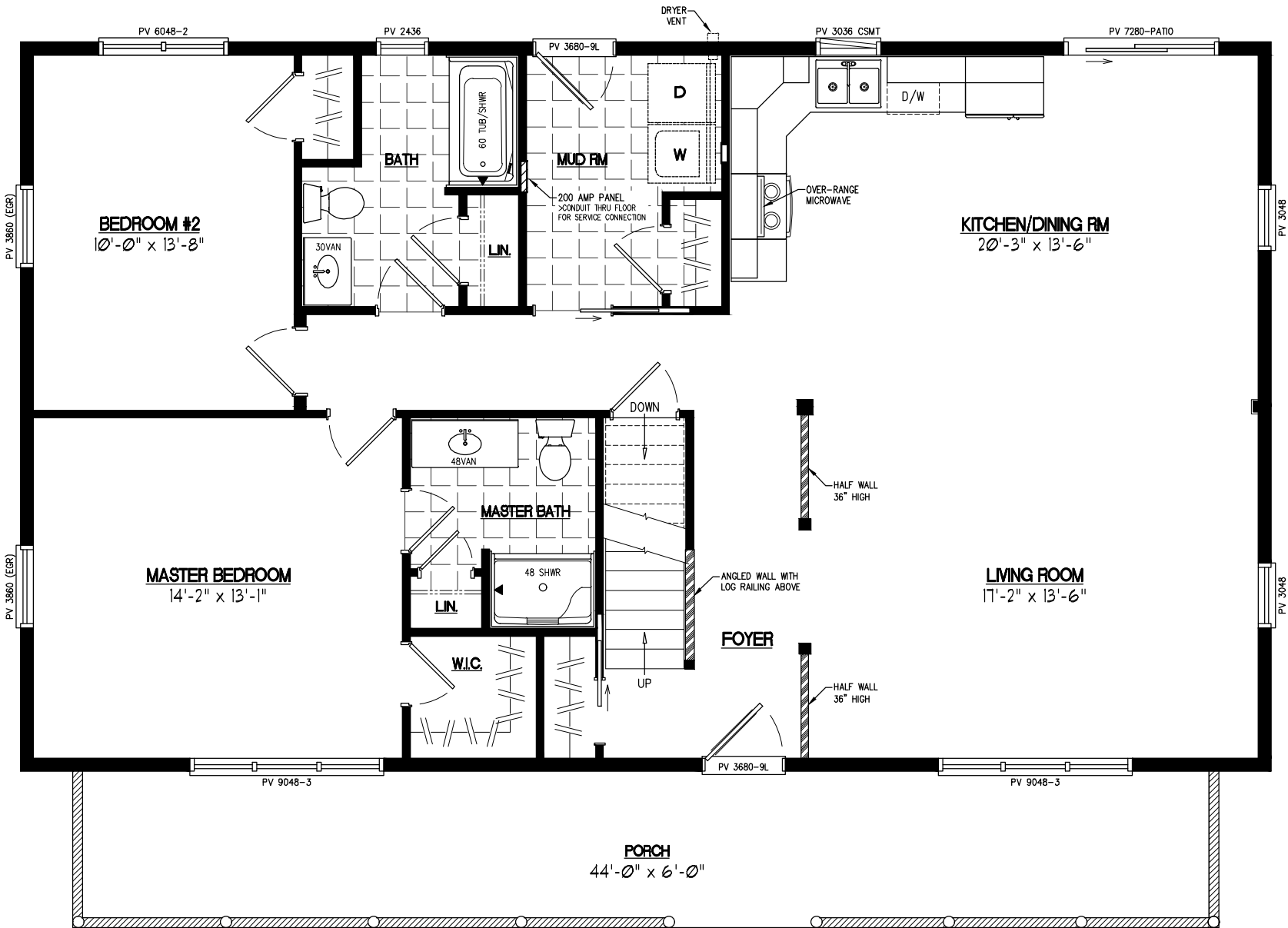
28x48 MOUNTAINEER Plan #28MR1305
