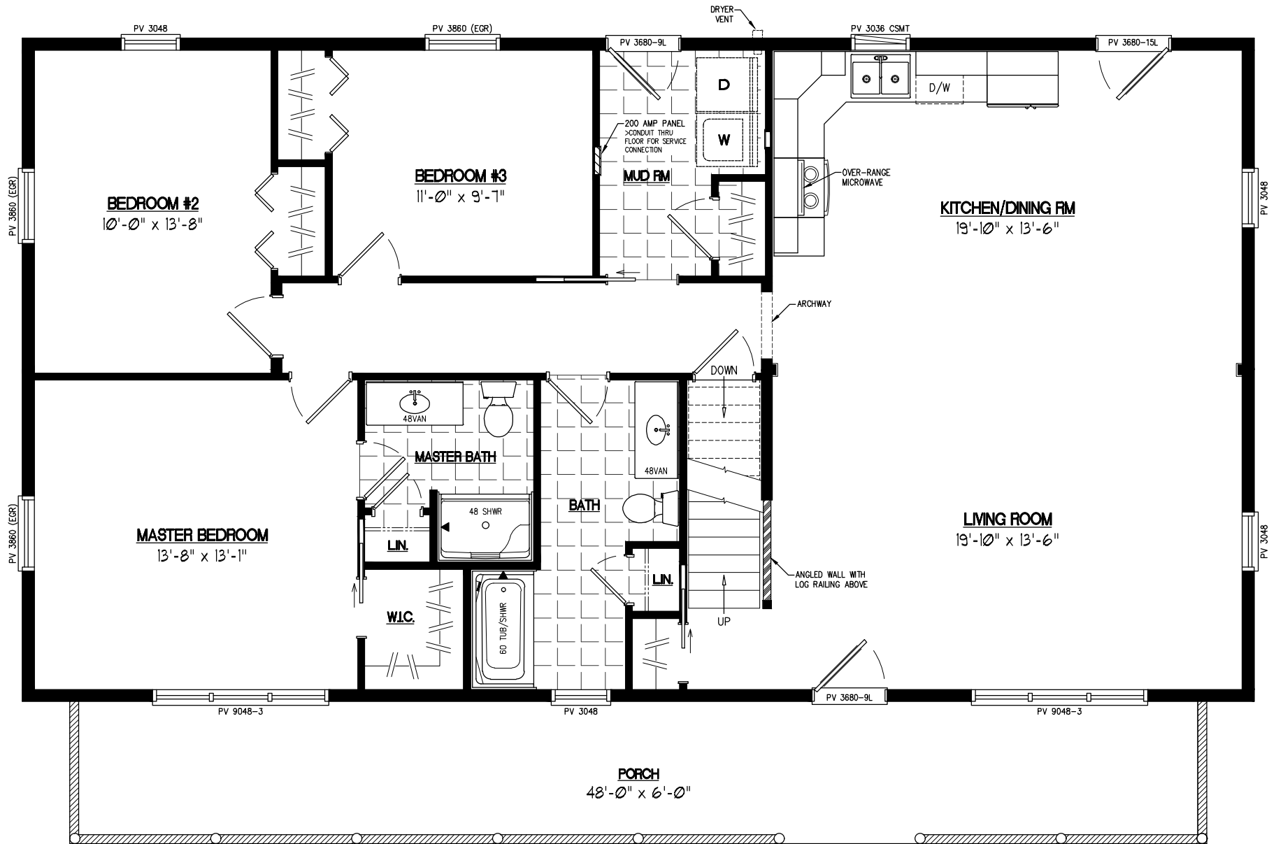
28x52 MOUNTAINEER Plan #28MR1307
