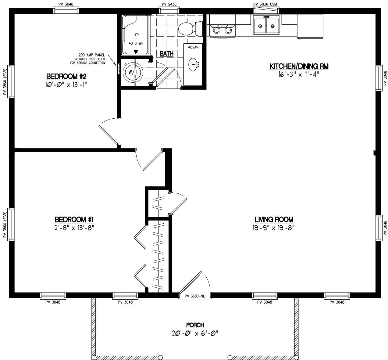
28x36 PIONEER Plan #28PR1202
