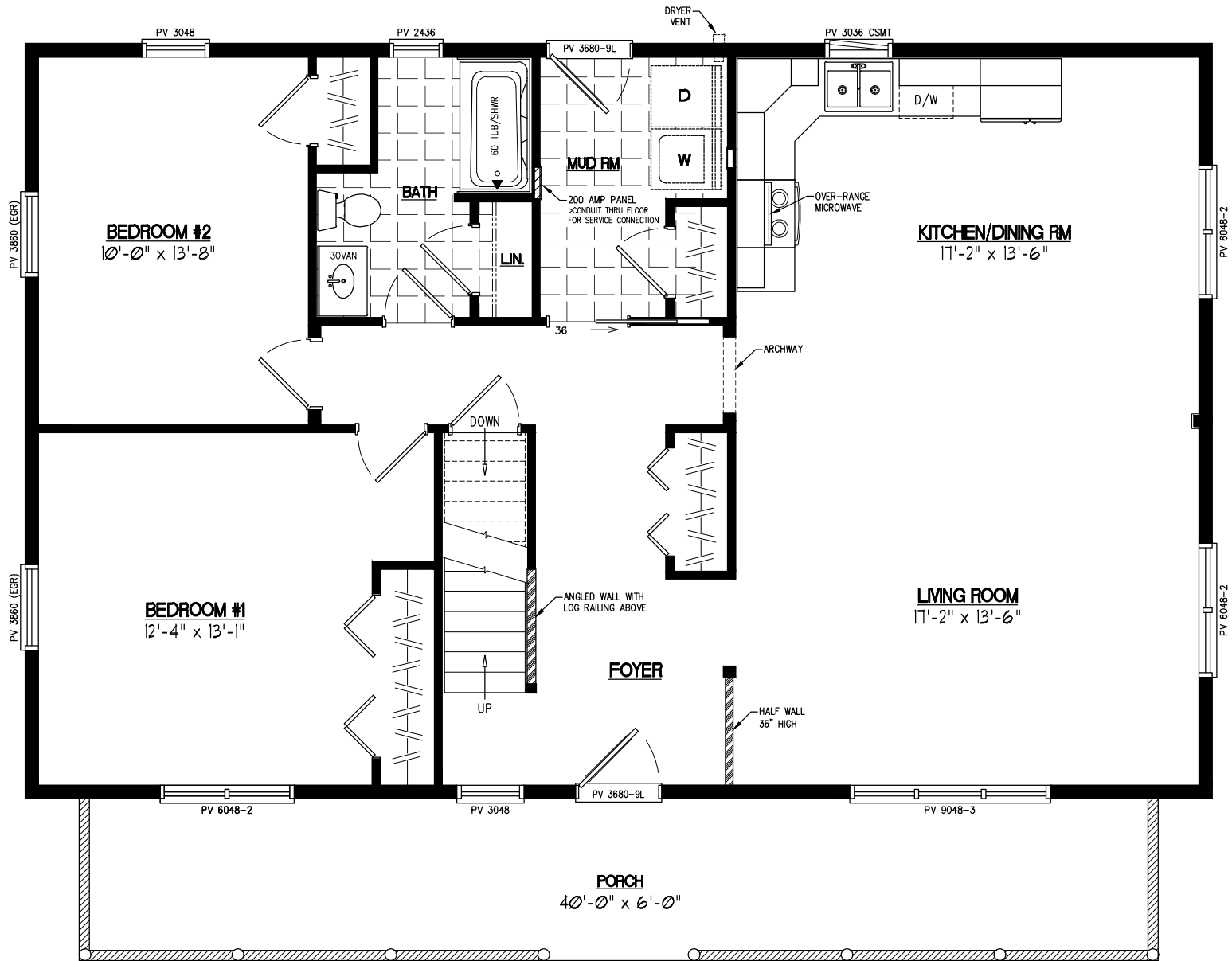
28x44 MOUNTAINEER Plan #28MR1304
