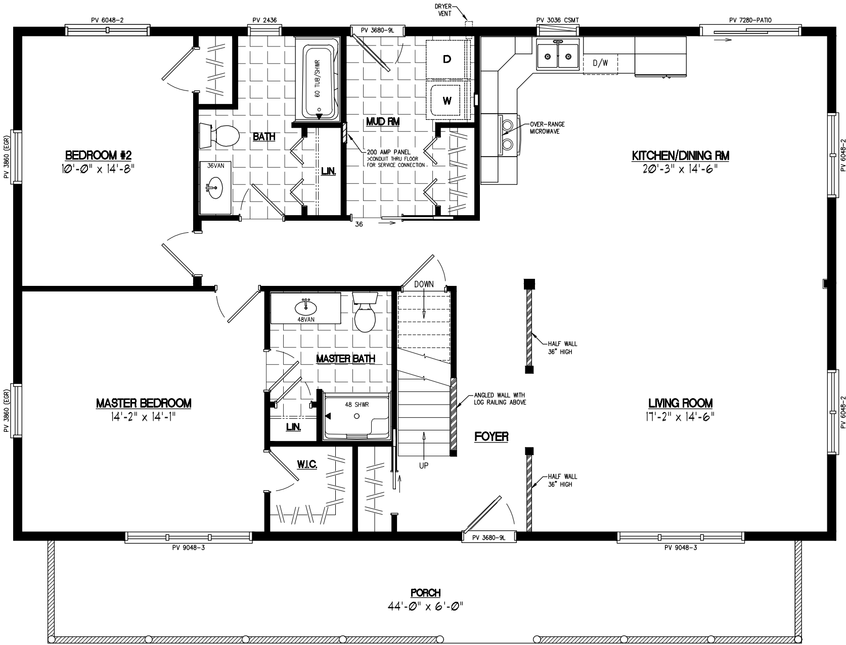
30x48 MOUNTAINEER Plan #30MR1305
